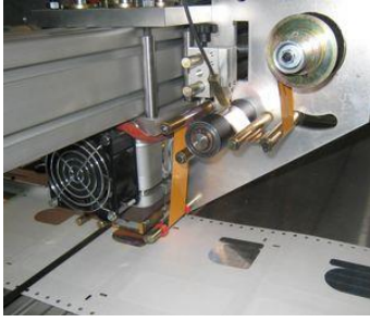
Hologram foil feeding system and stretching check at the printing unit.
